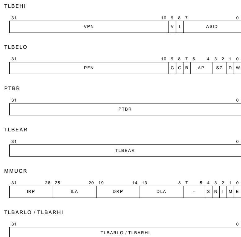
Figure 4-3. The MMU interface registers
