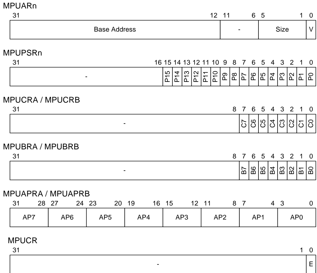
Figure 5-1. The MPU interface registers
