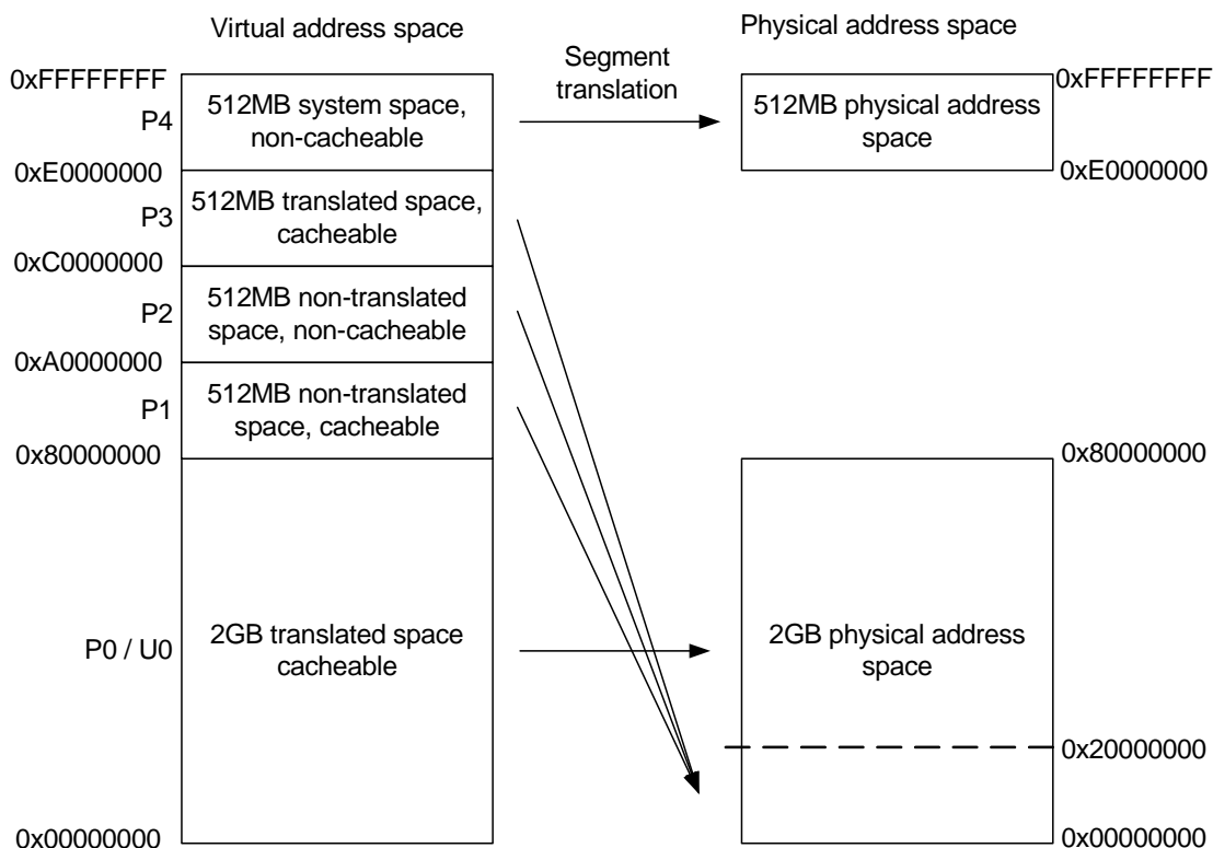
Figure 4-2. The AVR32 segment translation map
